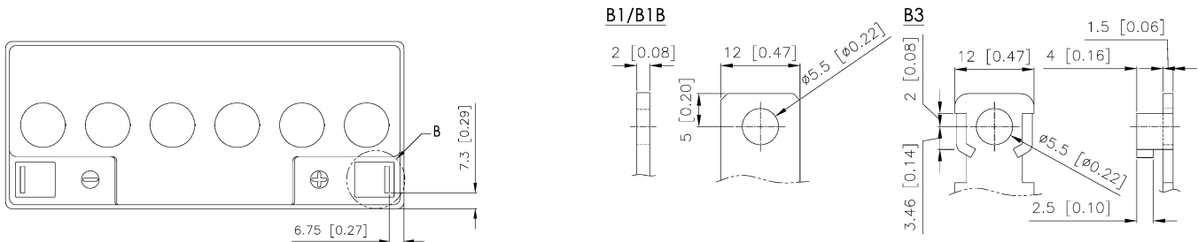
Detail B Drawing(1:1)
